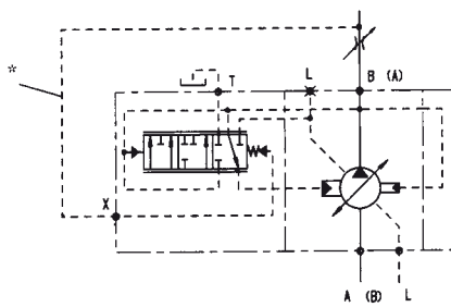
Flow compensation
