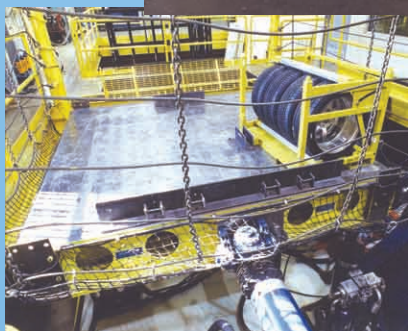
6 Axes Simulator
